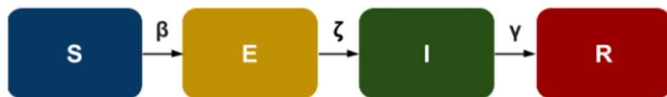
Figure 2: Compartmental model with four classes: S, E, I, and R. The parameters \beta , \zeta , and \gamma each represent flow rates between classes. In this diagram, \beta is the rate at which the susceptible become infected, \zeta is the rate at which the exposed move into the infectious class, and \gamma is the rate at which the infected are removed from the infectious class.
